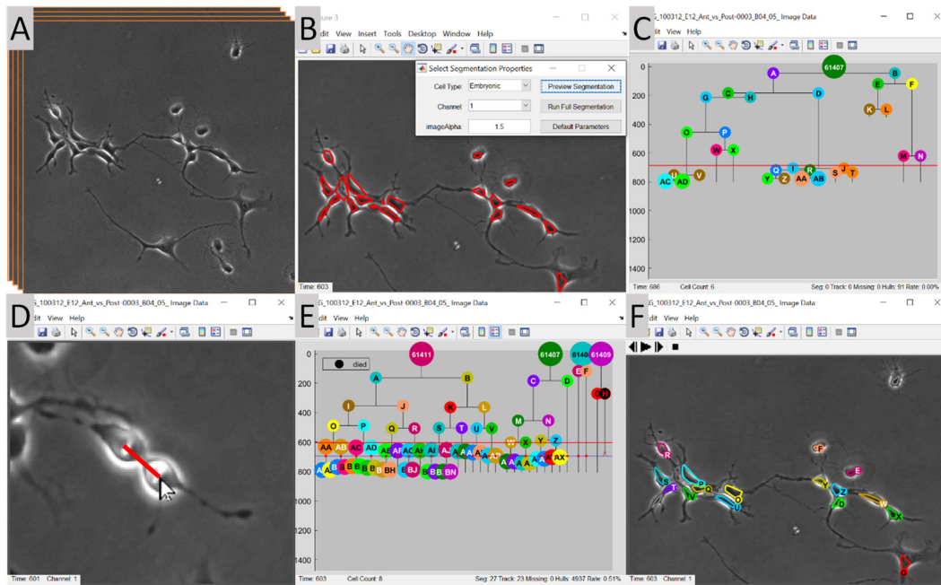
Figure 1. LEVER processing pipeline. Cells in the input image sequence (A) are automatically identified. Cell detection algorithms and parameters are tested on single image frames using the segmentation previewer (B). LEVER automatically creates an initial lineage tree based on cell tracking (C). The user quickly identifies all mitotic events to specify a corrected lineage tree in minutes (D). Using four interacting lineages (E) LEVER segmentation refinement can automatically correct most errors. Remaining errors are corrected manually during the refinement process (F).
